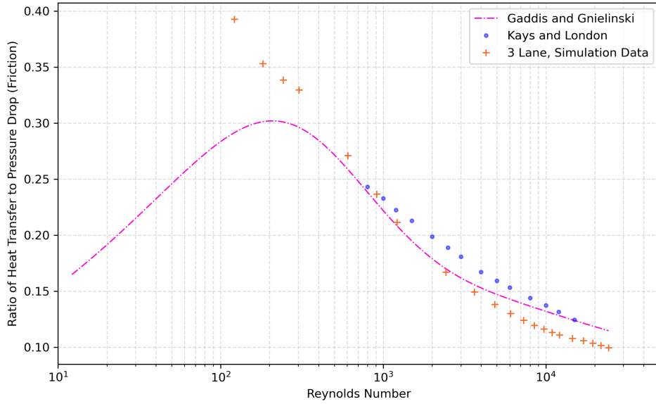
Figure 17: Ratio of heat transfer to pressure drop (friction) plot for staggered X_t^* = 1.5, X_\ell^* = 1.25 .
