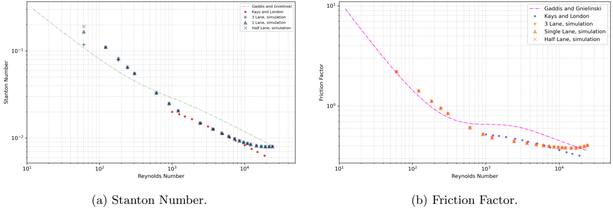
Figure 6: Comparison for staggered X_t^* = 1.5 , X_\ell^* = 1.25 against Kays & London and Gaddis & Gnielinski.
