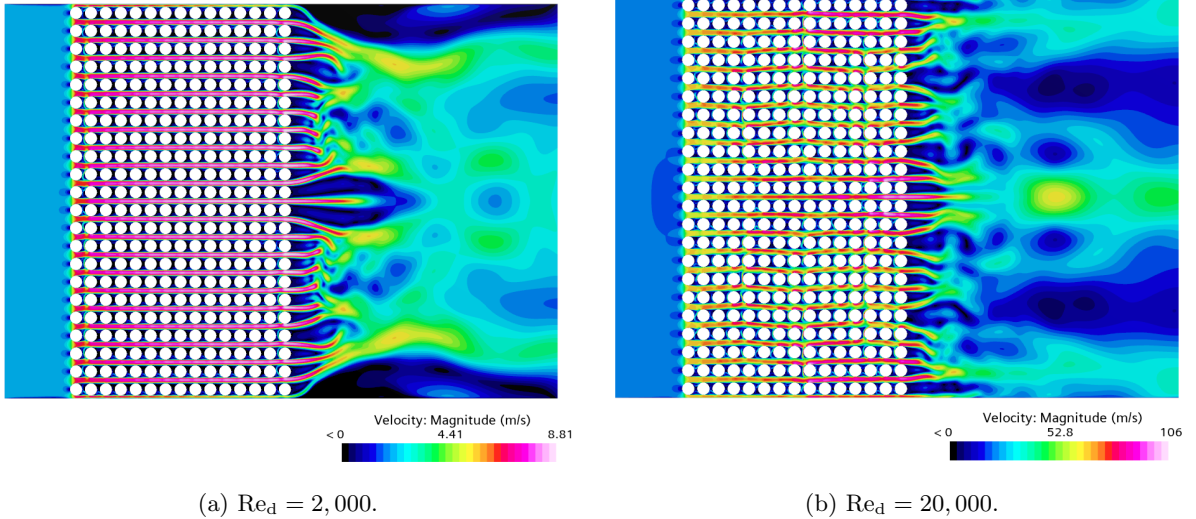
Figure 10: Velocity scenes for X_t^* = 1.5 , X_\ell^* = 1.25 inline tube bank.
