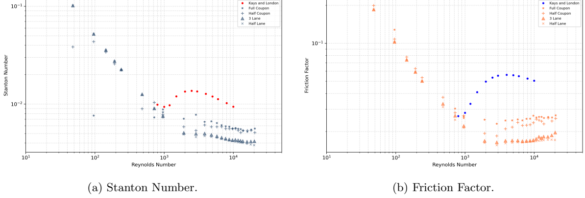
Figure 5: Comparison for inline X_t^* = 1.5 , X_\ell^* = 1.25 against Kays and London.
