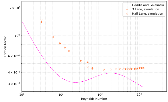
(b) Friction Factor.
