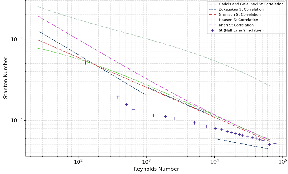
Figure 9: Comparison for inline X_t^* = X_\ell^* = 2 against various correlations.
