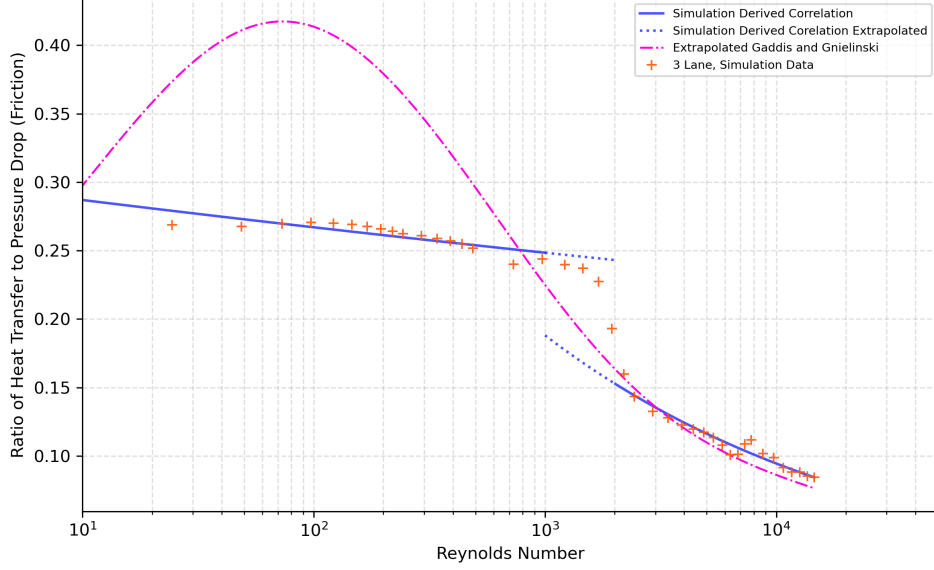
Figure 18: Ratio of heat transfer to pressure drop (friction) plot for inline X_t^* = 6 , X_\ell^* = 1.25 .
