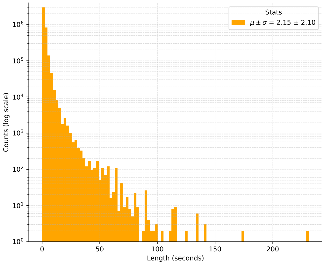
Segment Length Distribution (Multiplicative, \tau = 2.1 )
