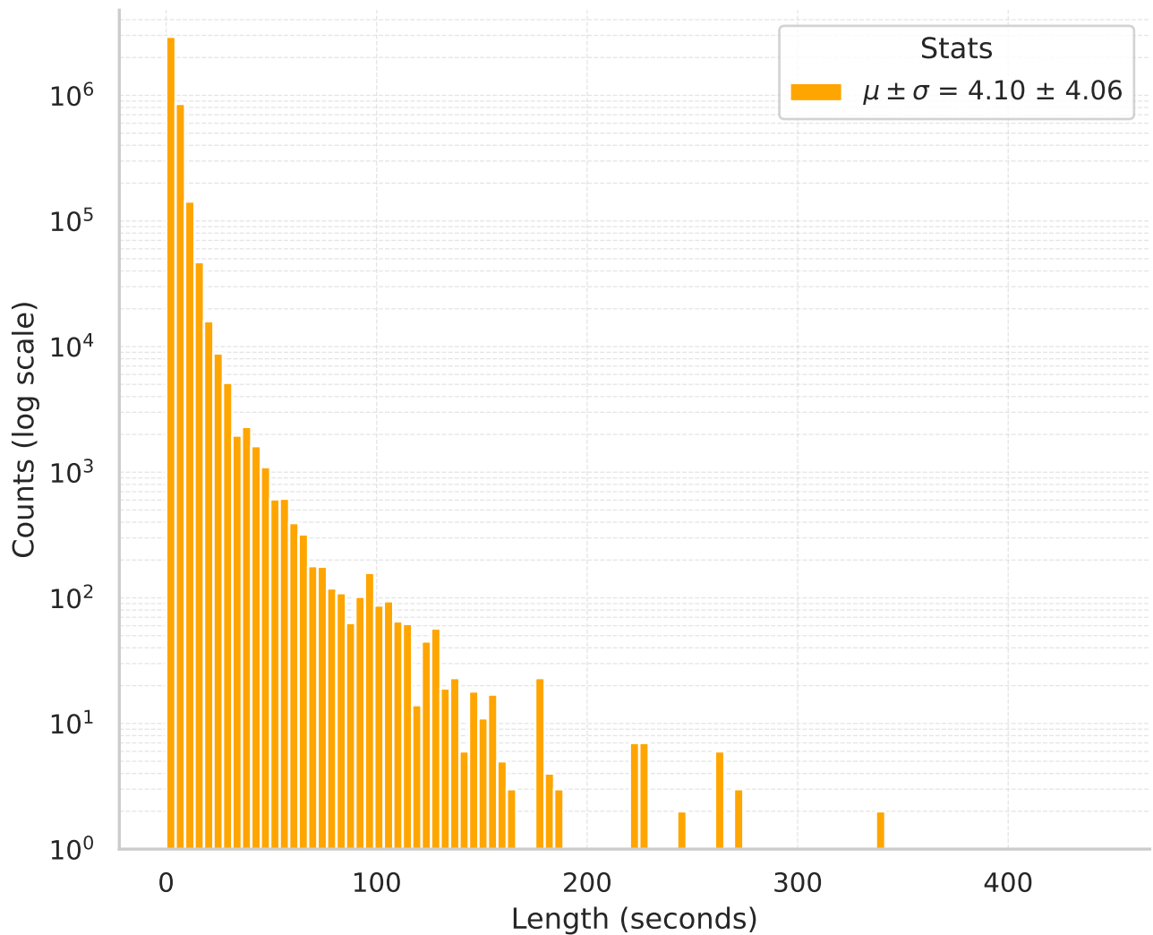
Segment Length Distribution (NLQ, S = 5 )
