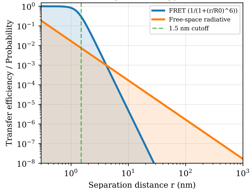
(a) Two-regime energy transfer
