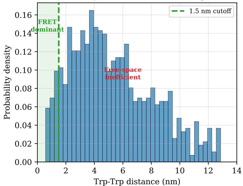
(b) PDB pair distances (4 targets)
