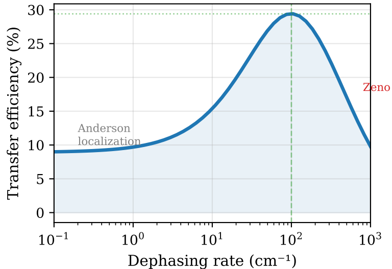
(a) ENAQT with static disorder
