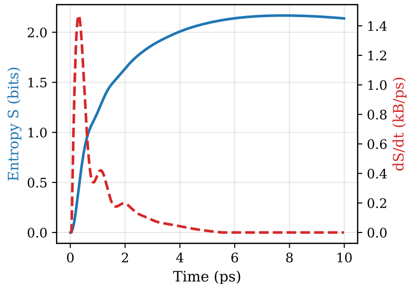
(a) Entropy trajectory at \gamma=100\text{ cm}^{-1}
