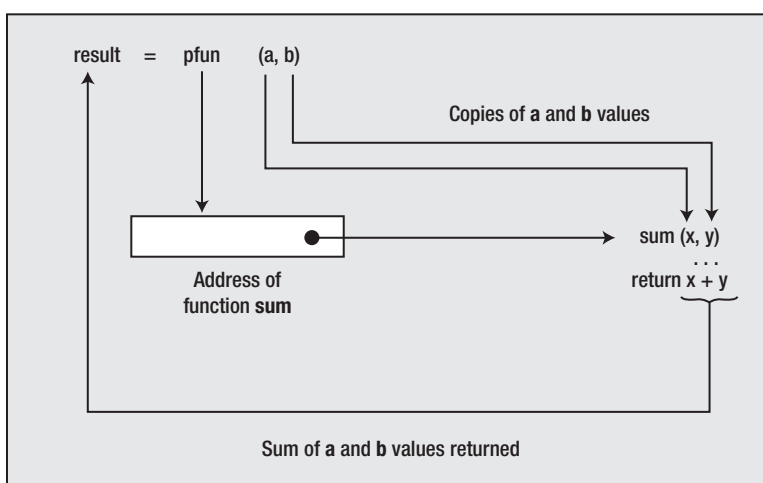
Figure 9-2. Calling a function through a pointer
