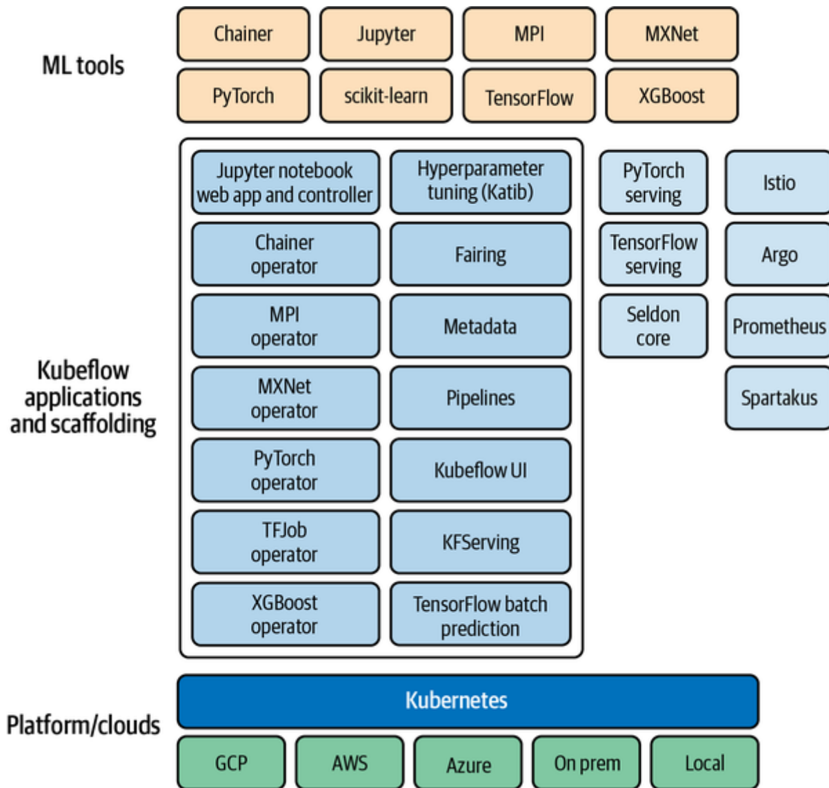
Figure 9-6. Kubeflow architecture
