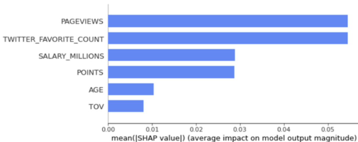
Figure 5-44. SHAP feature importance
