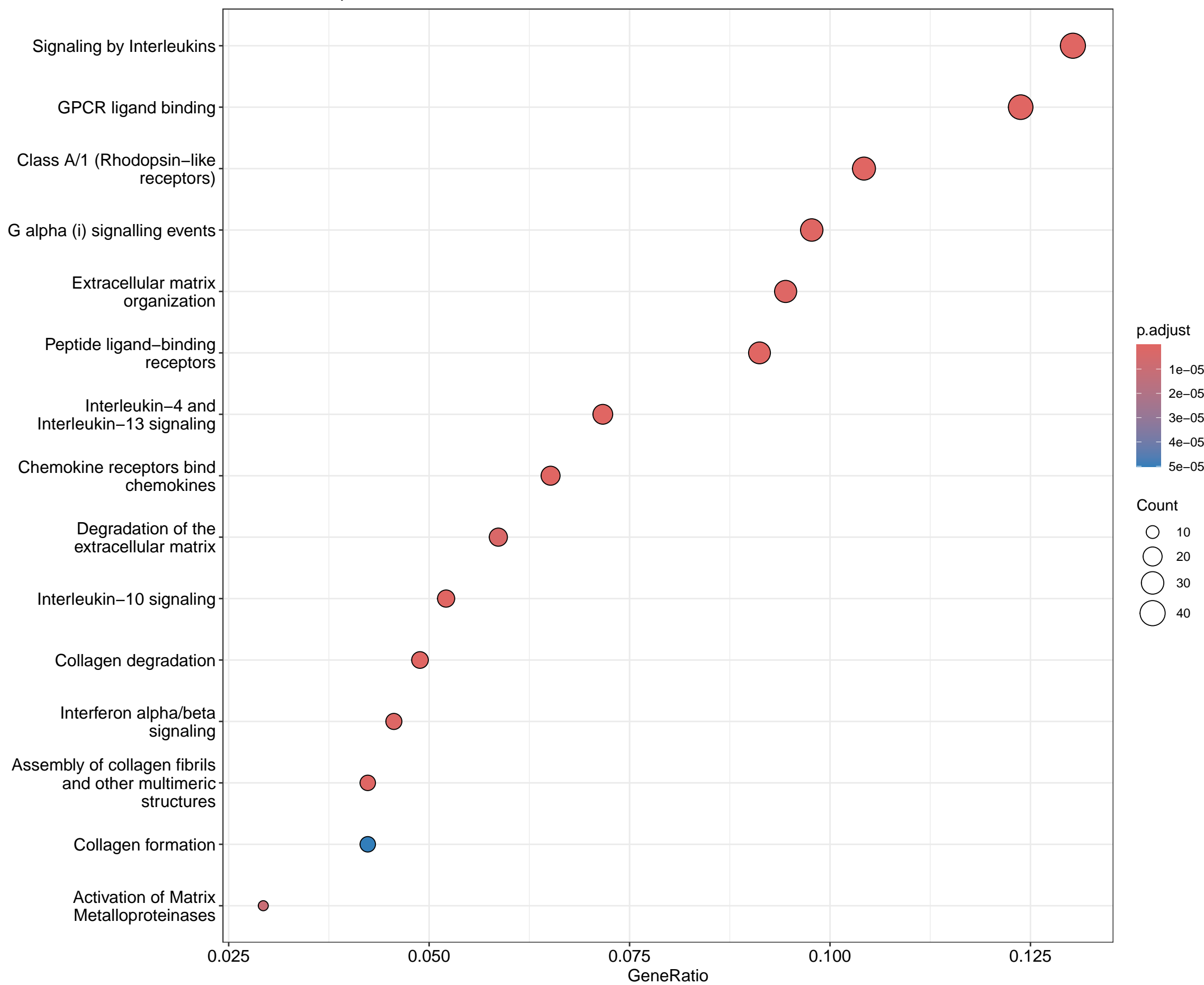
Reactome Dotplot
