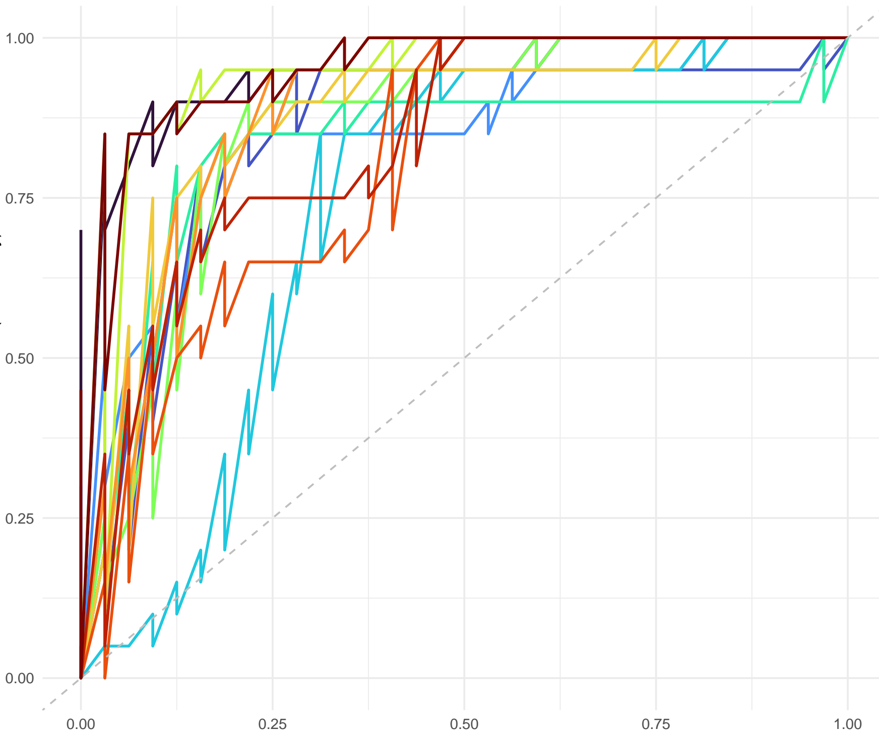
ROC Curves for Hub Genes: HC_vs_LSC
