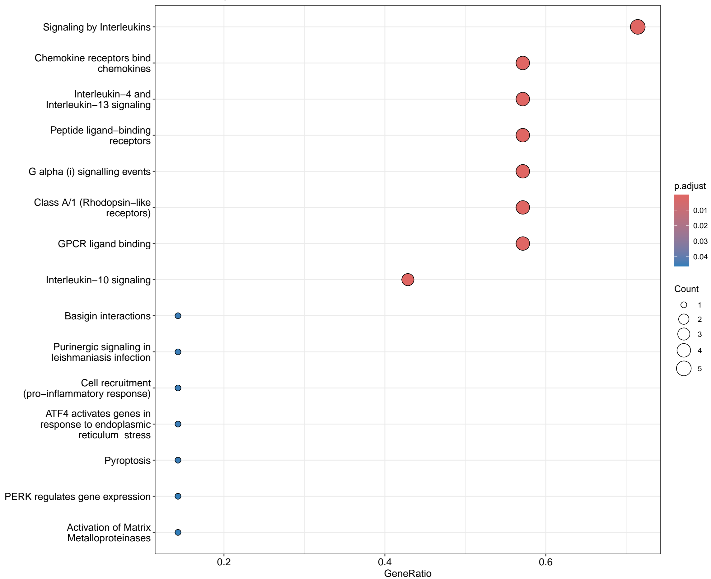
Reactome Dotplot
