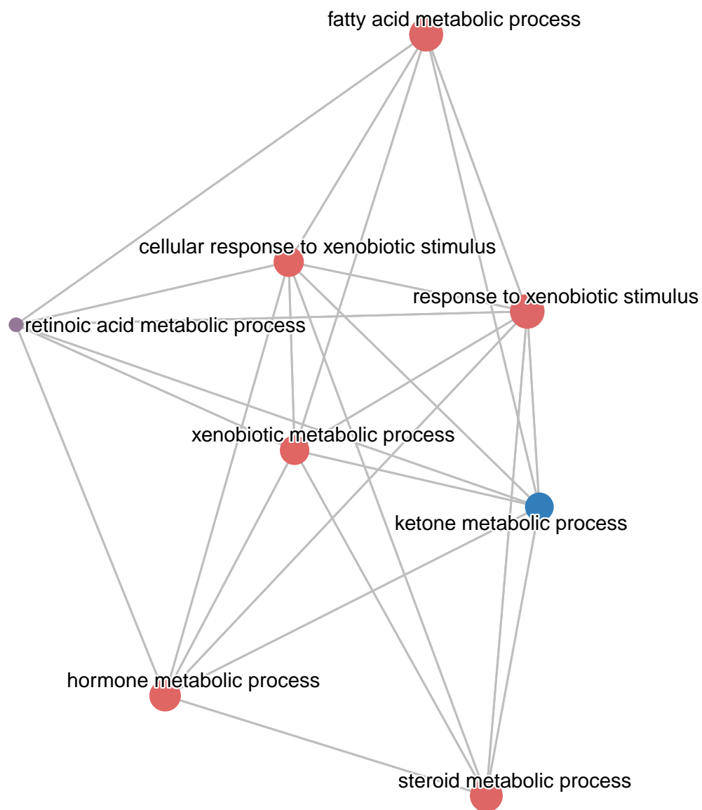
Enriched BP emapplot
