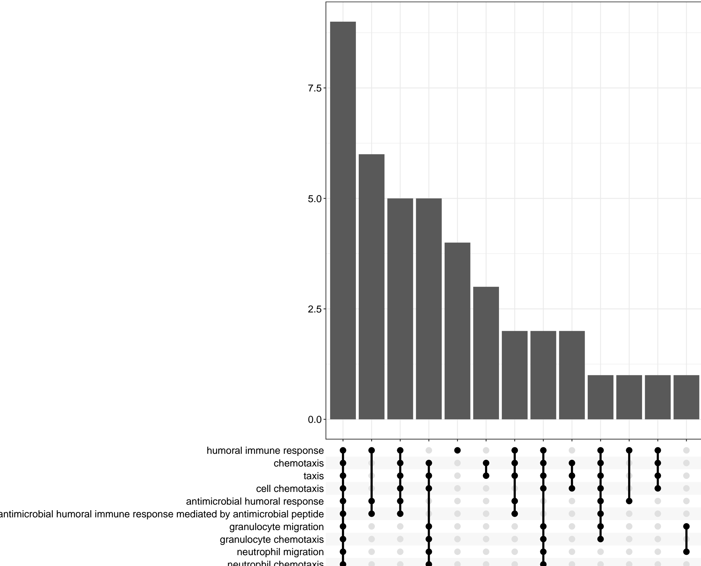
UpSet Plot of BH
