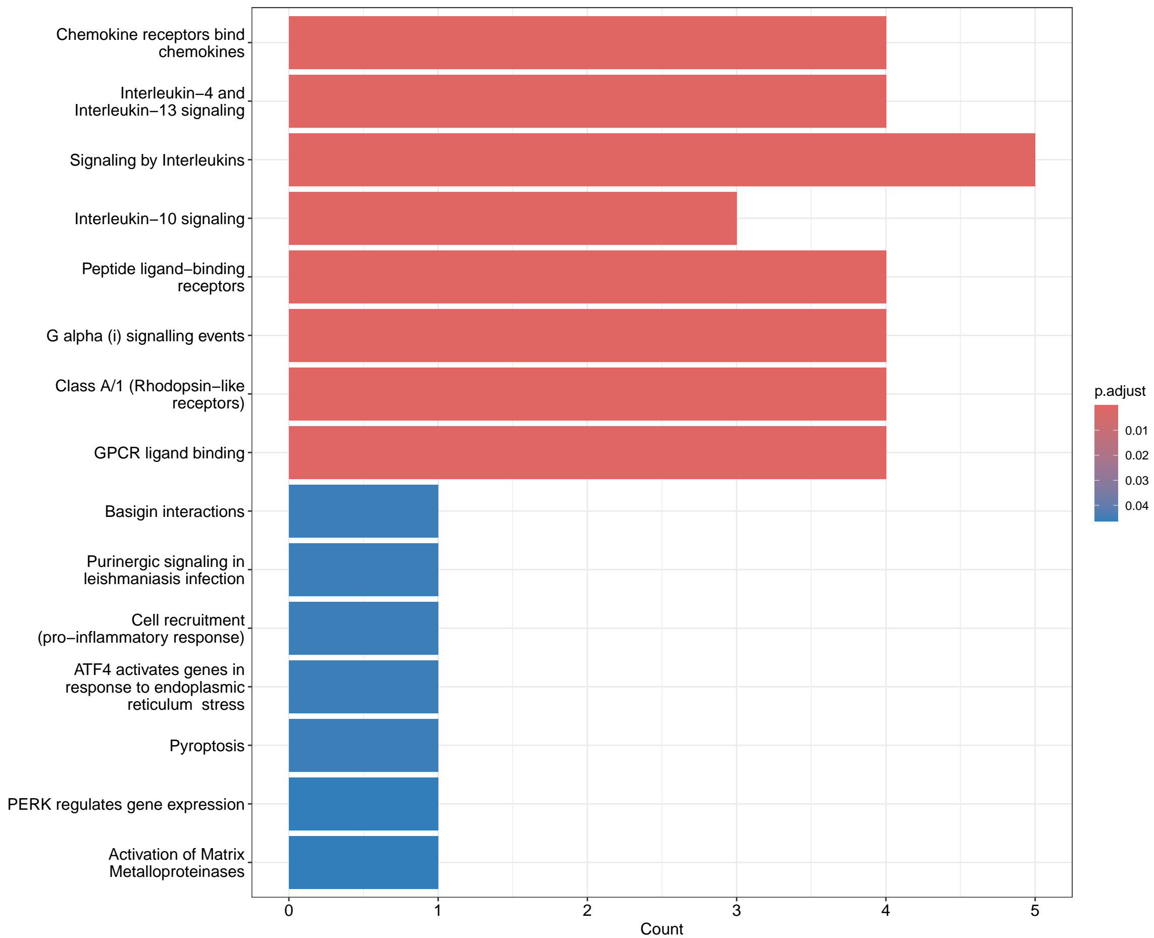
Reactome Barplot
