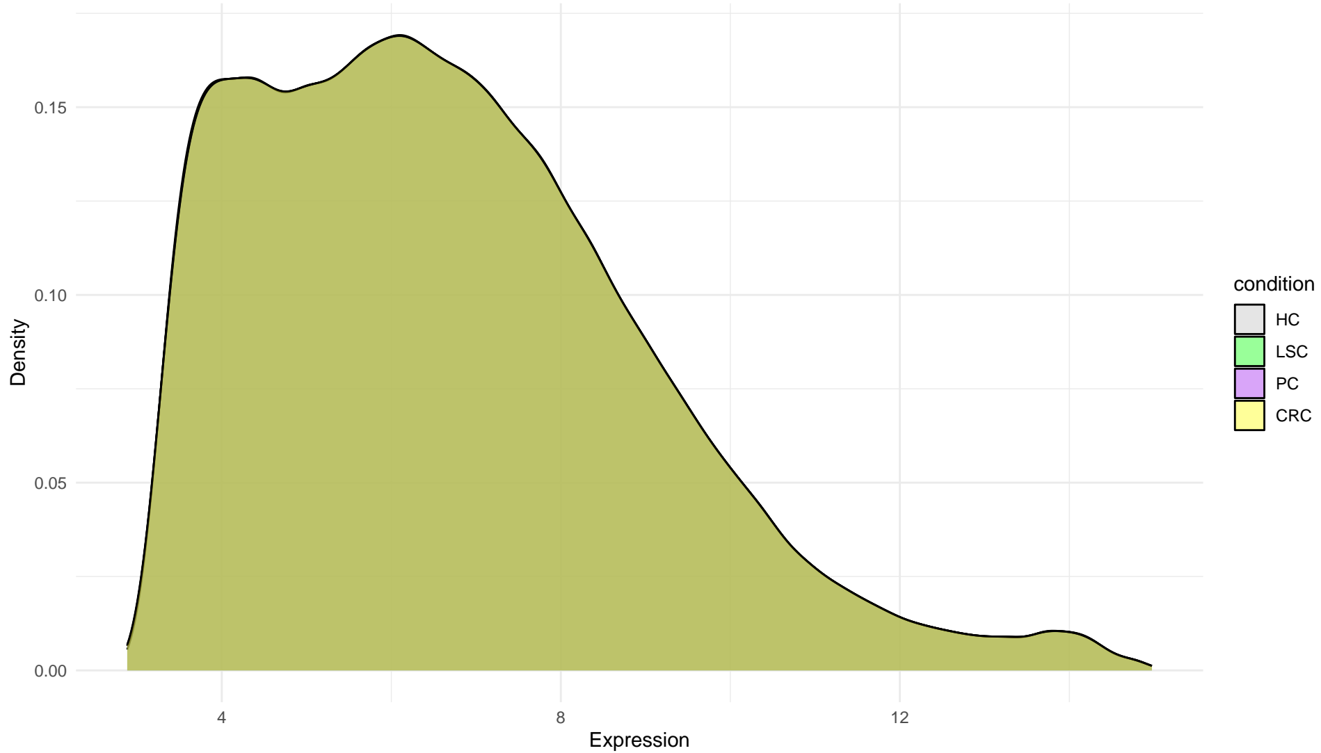
Expression Distribution of Noramlized expression data
