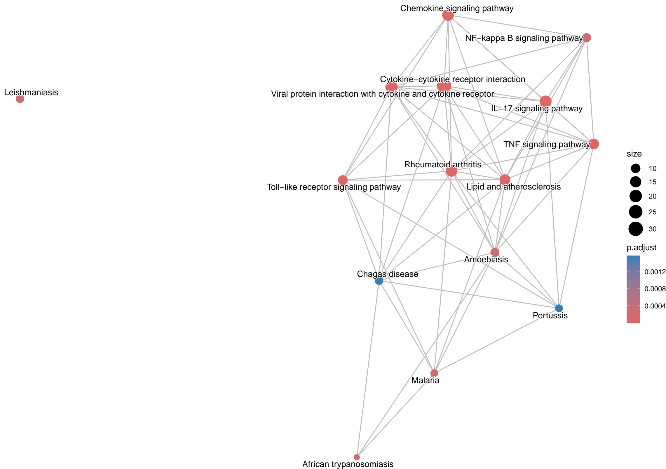
Enriched KEGG emapplot
