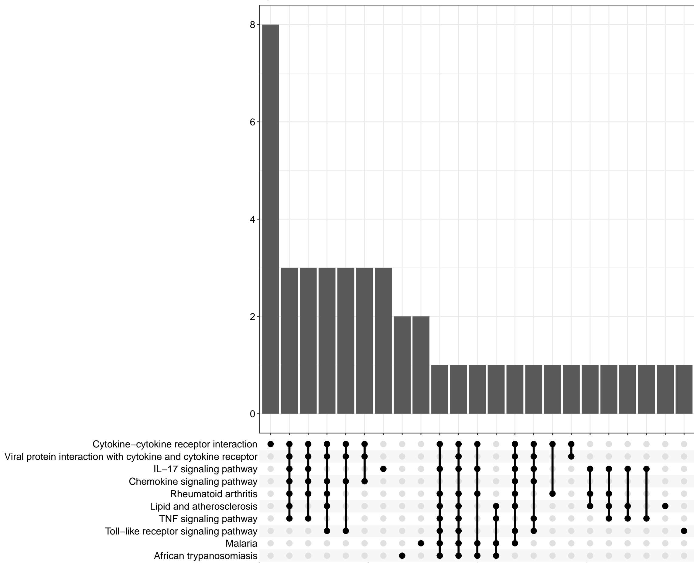
UpSet Plot of KEGG
