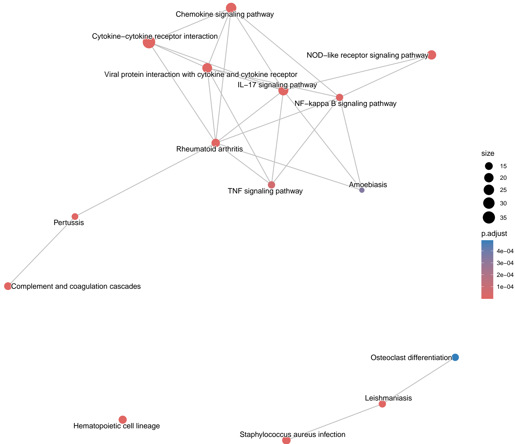
Enriched KEGG mapplot
