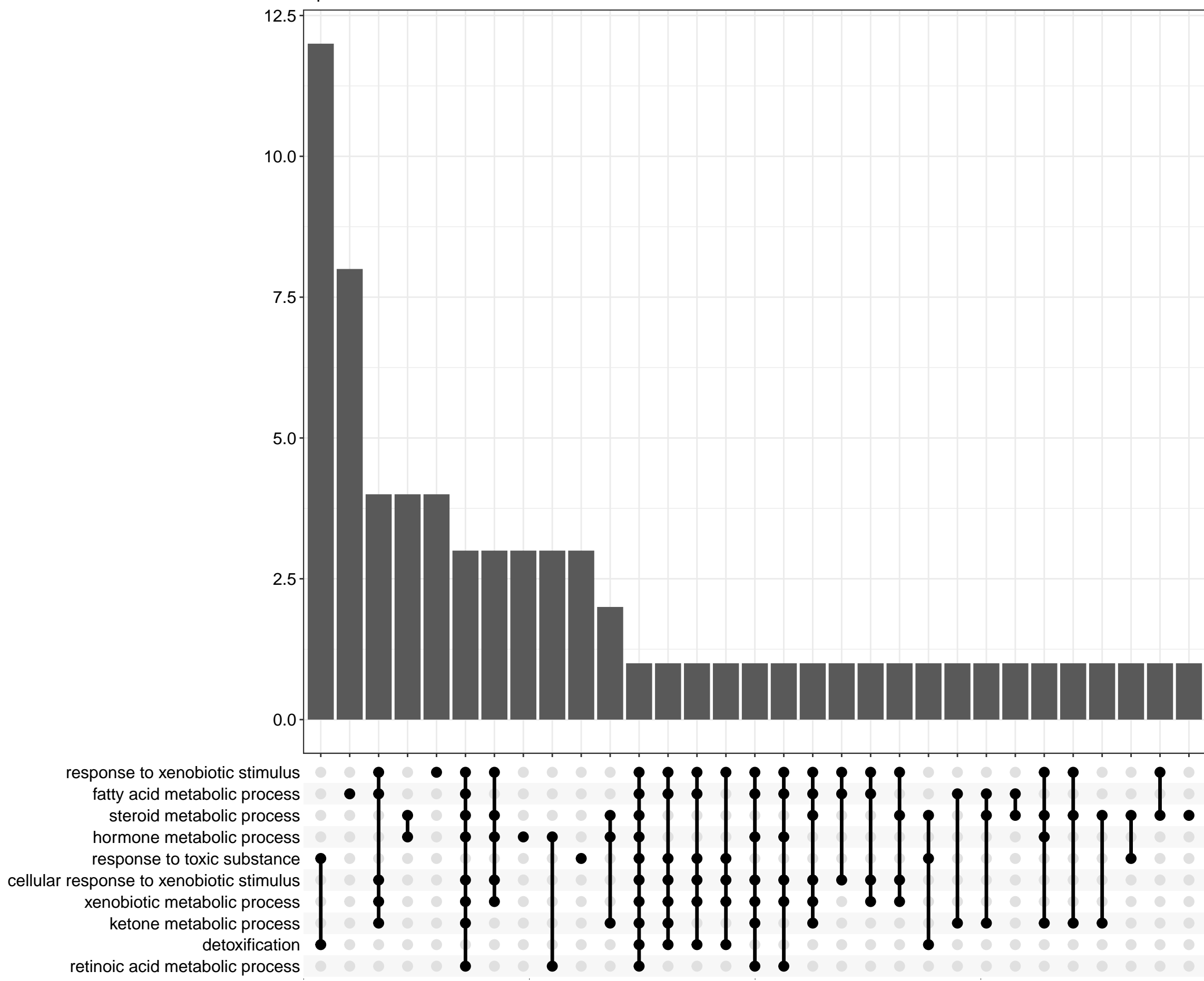
UpSet Plot of BP
