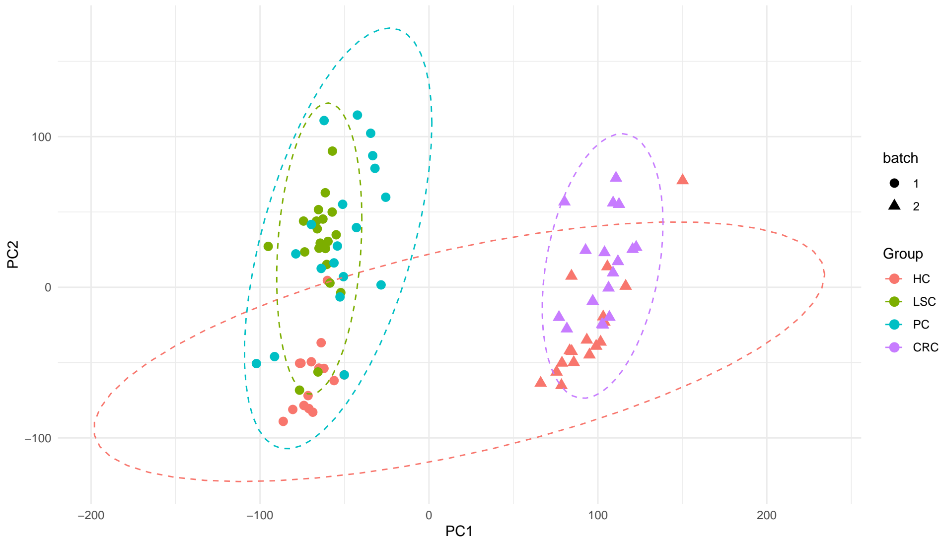
PCA of Normalized Expression Data
