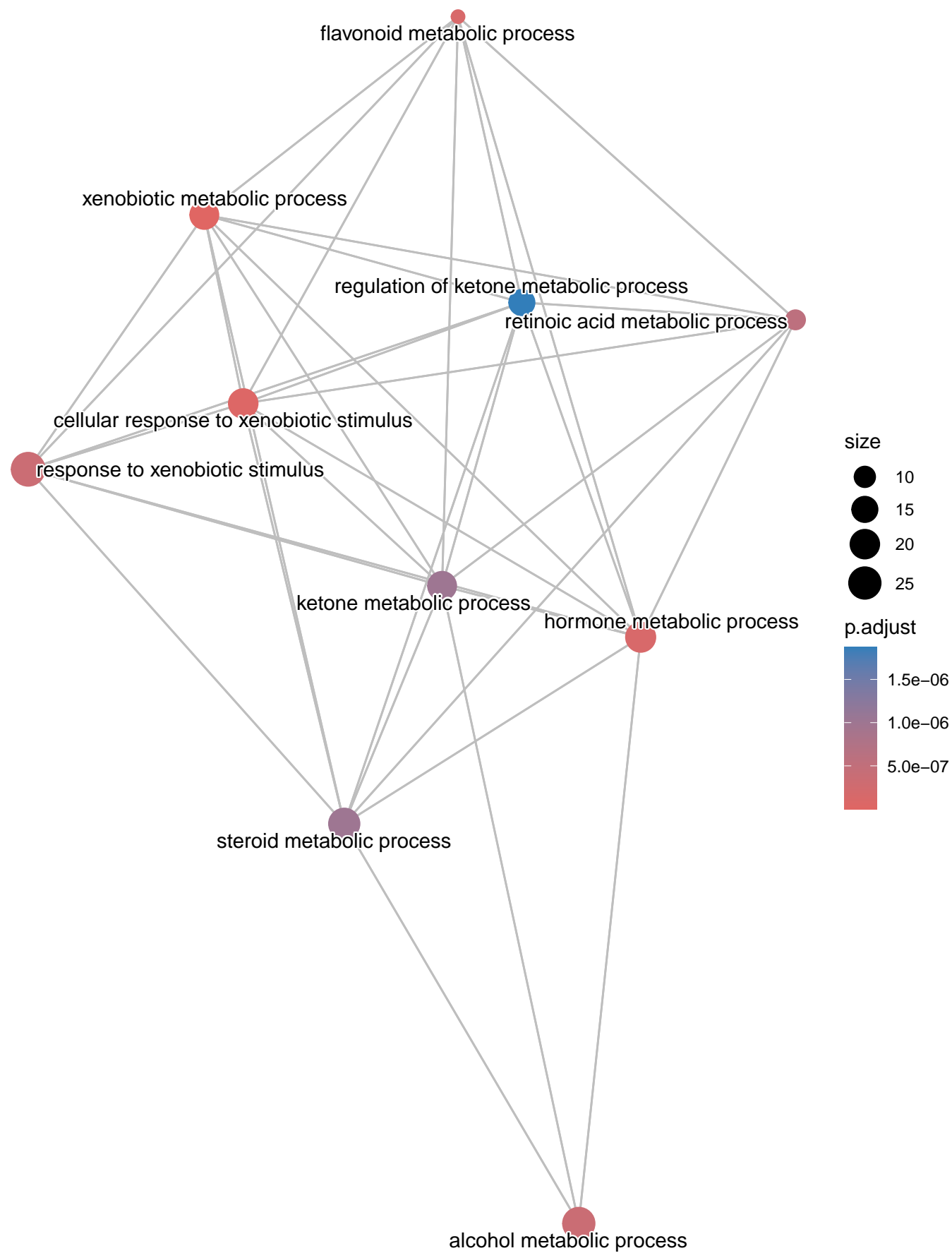
Enriched BP emapplot
