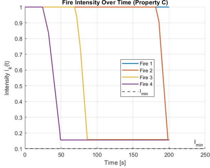
Figure 8: Multiple fires: Fire intensities over time.
