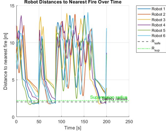
Figure 6: Multiple fires: Robot distance to nearest fire.
