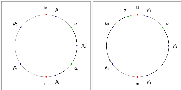
Figure 14: Some cases of c(k) .
