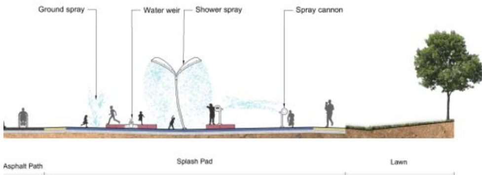
Figure 5: Ross Park spray park section
