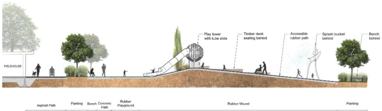
Figure 4: Ross Park fieldhouse and playground section
