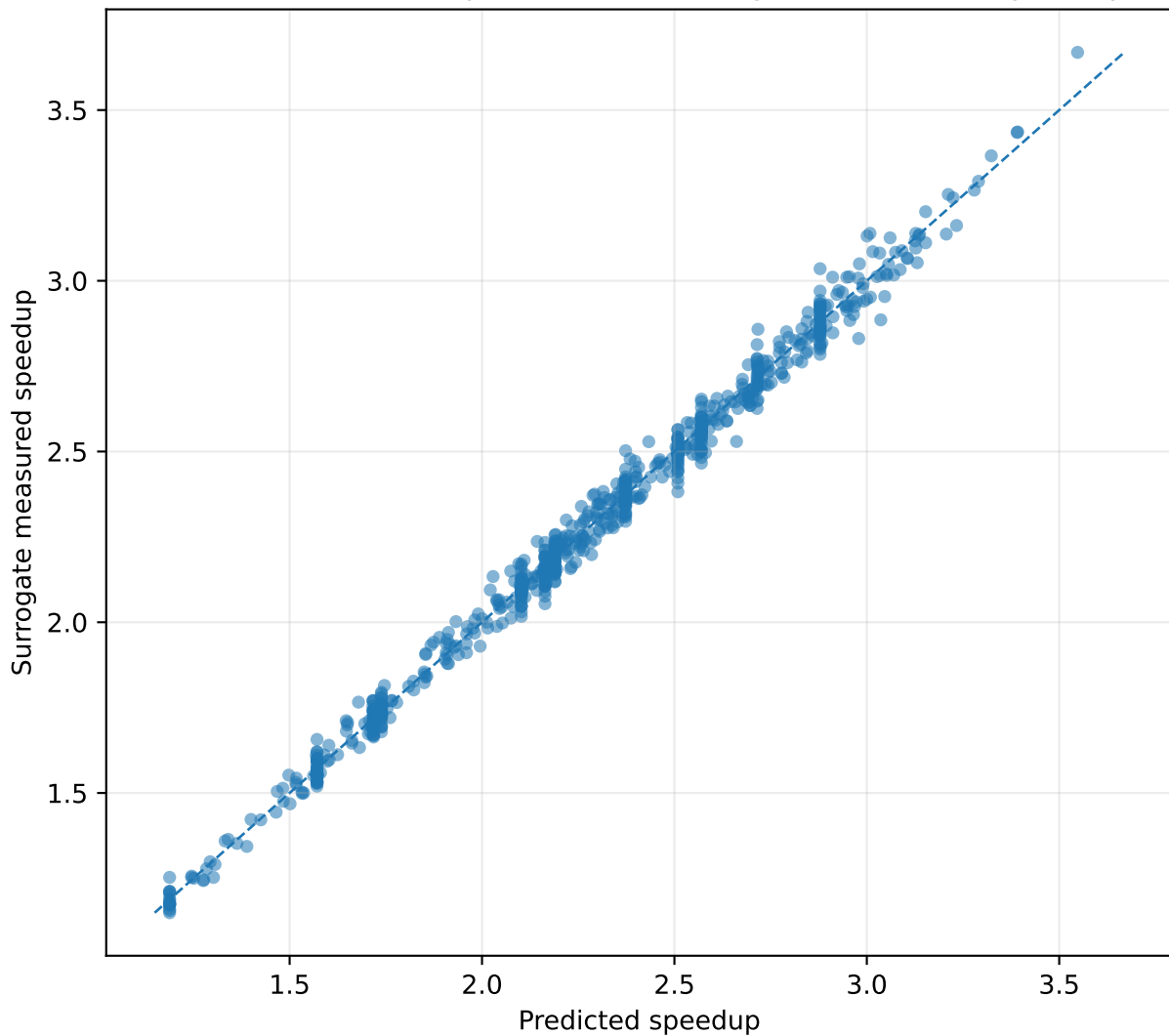
Runtime validation: predicted vs surrogate measured speedup
