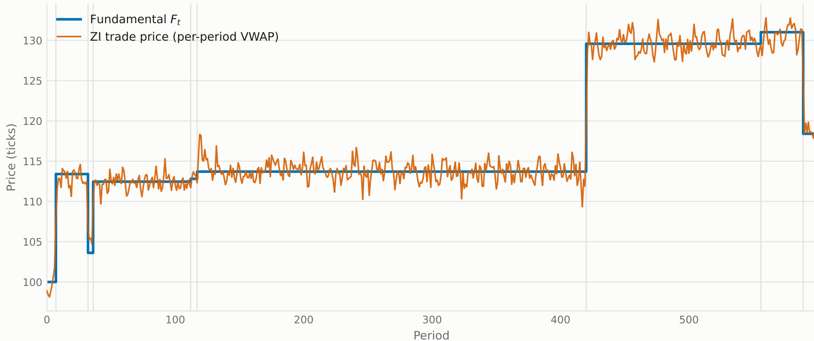
Zero-intelligence traders chase a jumping fundamental (40 traders, seed 7, 8 jumps)
