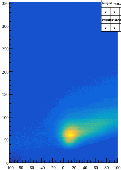
Subtracted
