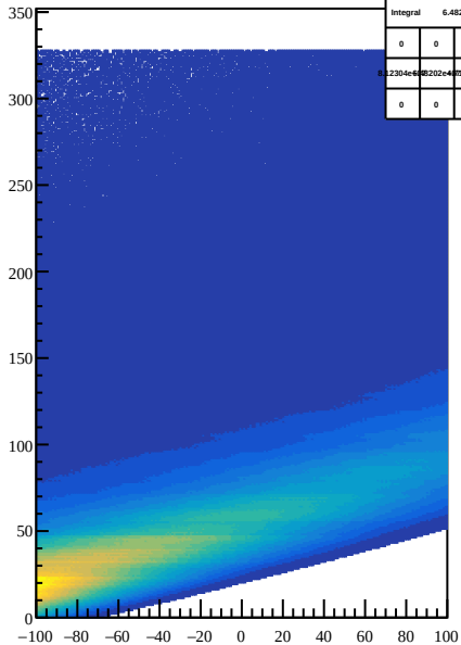
Random
