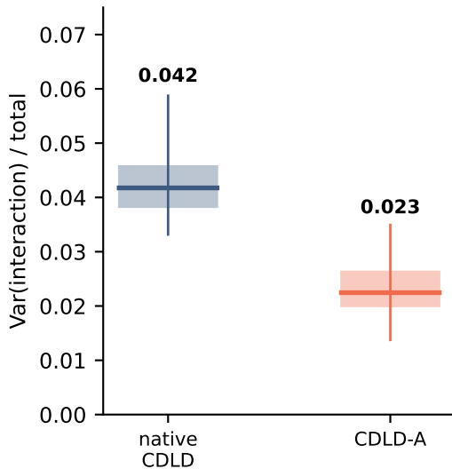
(b) decomposition of the fitted function — prespecified
