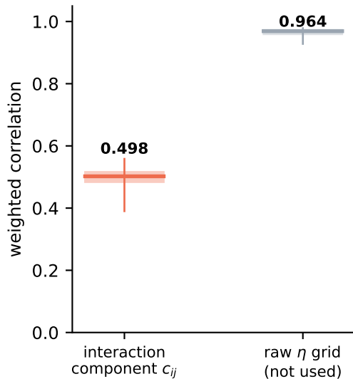
(c) do the two models find the same interaction structure?
