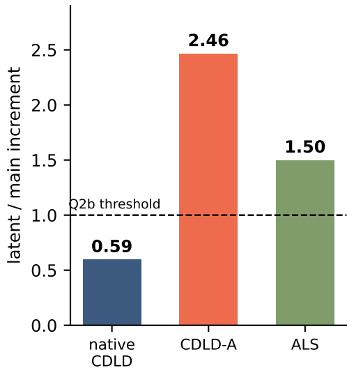
(a) decomposition of predictive skill (Q2b)
