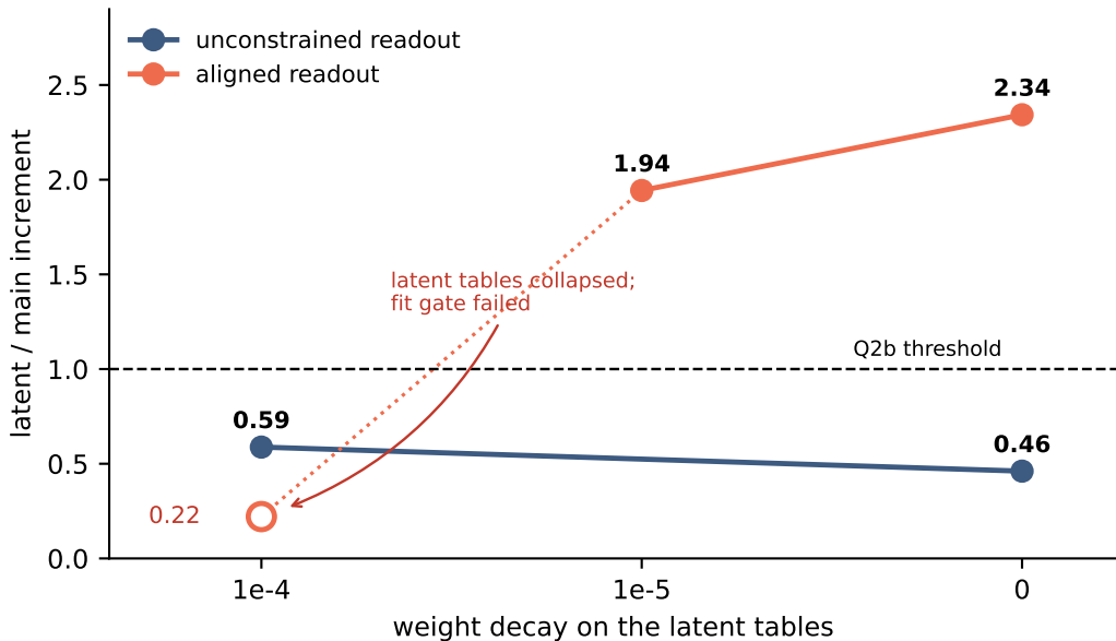
The ratio classification remains separated after varying latent-table regularisation
