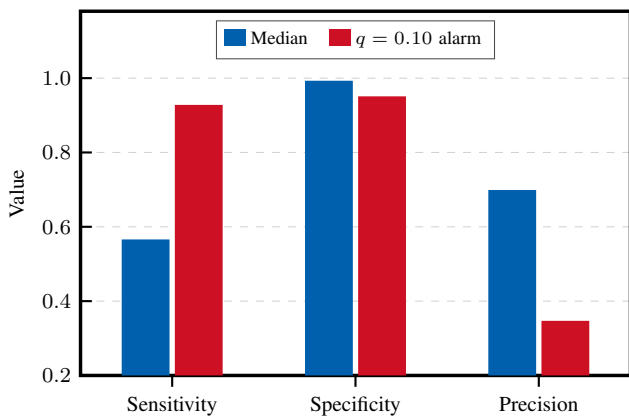
Fig. 6. Hypoglycemia alarm trade-off at 30 minutes comparing the median forecast with the q = 0.10 lower-quantile alarm. The quantile alarm increases sensitivity from 0.566 to 0.928 with little change in specificity, but reduces precision from 0.699 to 0.347 due to more frequent false alarms. This represents a tunable sensitivity-precision trade-off, not deployment readiness.
