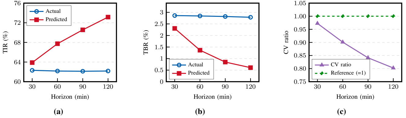
Fig. 7. Excursion compression with horizon (30/60/90/120 minutes). 7a: actual time-in-range (TIR) stays flat near 62% while predicted TIR climbs toward 74%, an increasing overestimate. 7b: actual time-below-range (TBR) stays flat near 2.8% while predicted TBR falls toward 0.6%, an increasing underestimate of hypoglycemic exposure. 7c: the predicted-to-actual coefficient-of-variation ratio declines from about 0.97 to 0.80. All three panels show the same mechanism: as the horizon lengthens, the point forecast increasingly regresses toward the mean and loses the variance of the true glucose trace.
