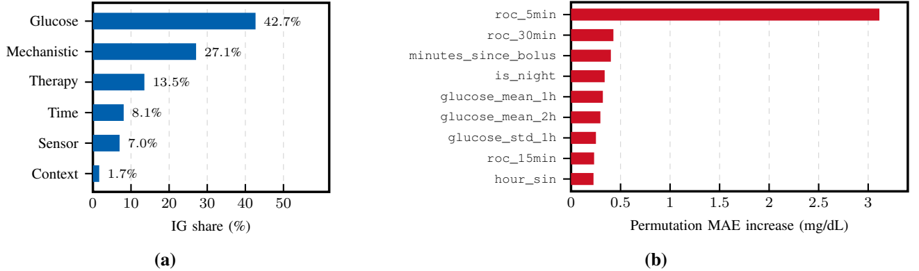
Fig. 8. Feature attribution at 30 min using integrated gradients (8a) and permutation importance (8b). Glucose-derived features dominate IG attribution (42.7%), while roc_5 is the strongest permuted feature ( \sim 3.1 mg/dL MAE increase). Both methods identify glucose dynamics as the leading predictors.
