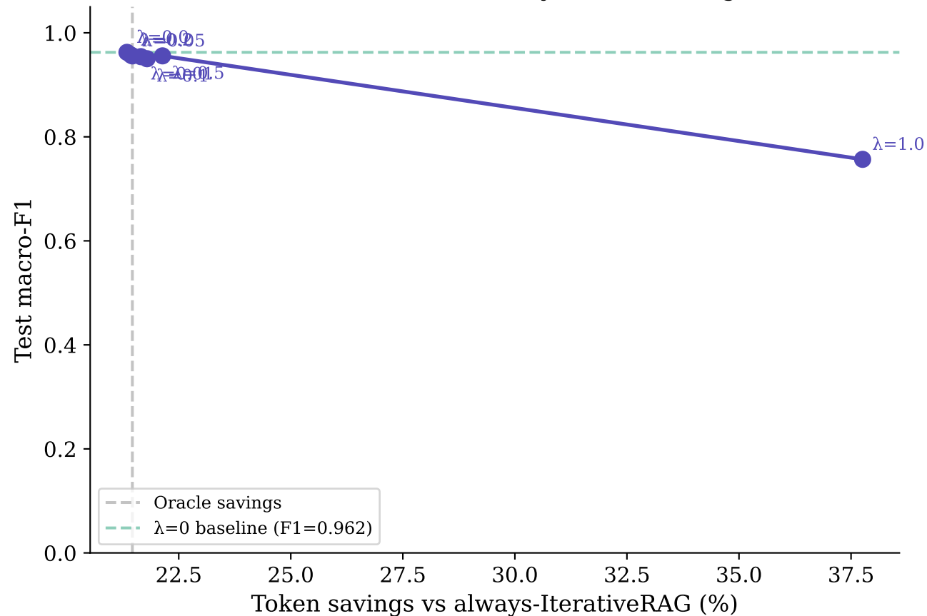
Pareto frontier: accuracy vs cost savings
