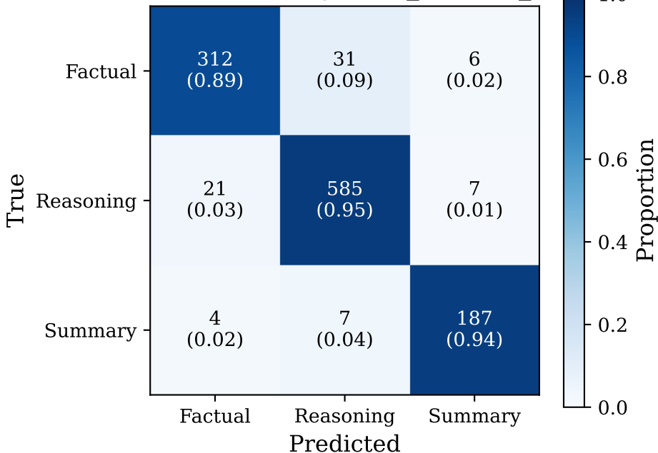
Confusion Matrix: TinyBERT_General_4L_312D
