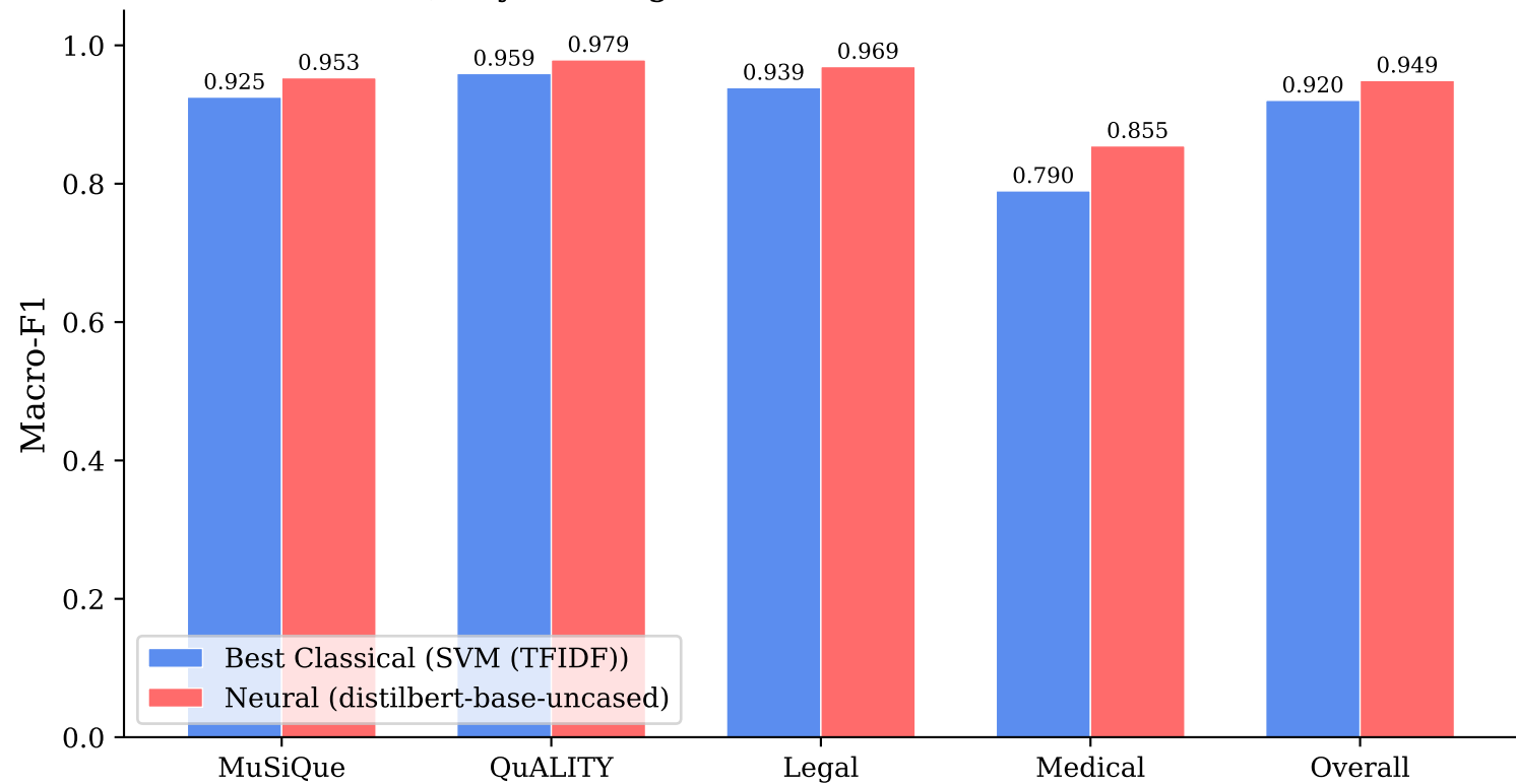
Query Routing: Classical vs Neural Classifiers
