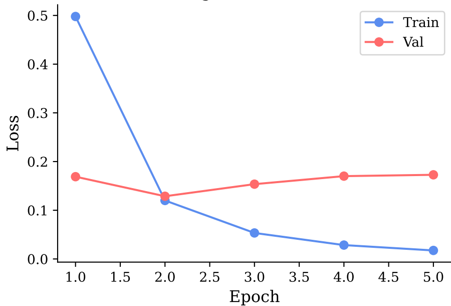
Training & Validation Loss
