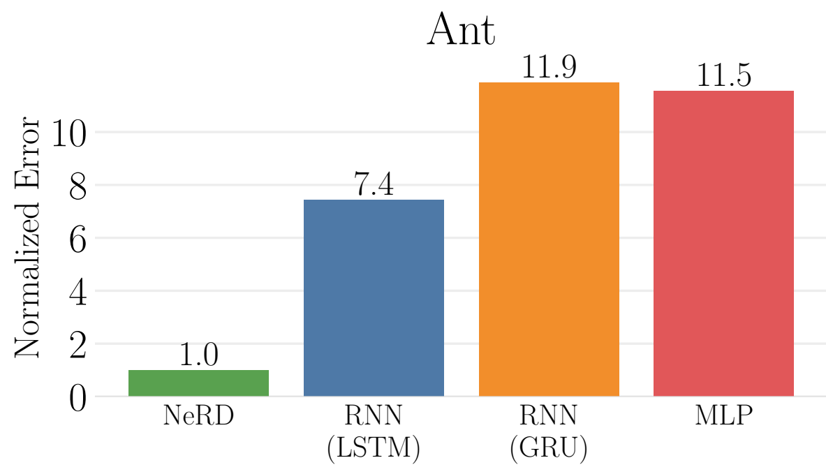
(a) Ablations on Neural Network Models
