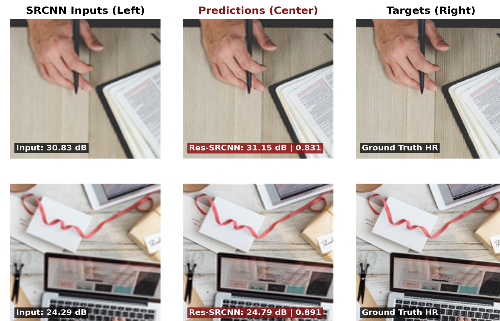
Figure 7: SRCNN inputs (left), predictions (center), targets (right)
