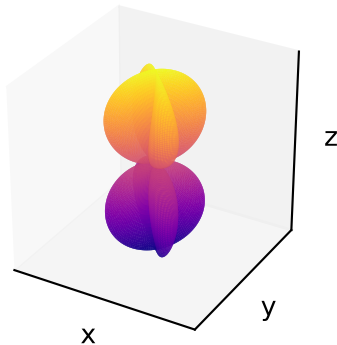
× Polarization
