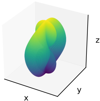
+ Polarization
