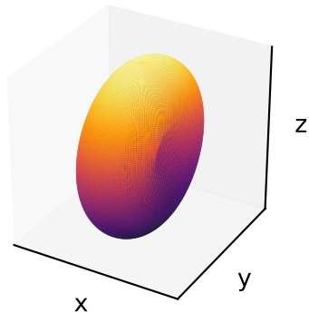
RMS Polarization
