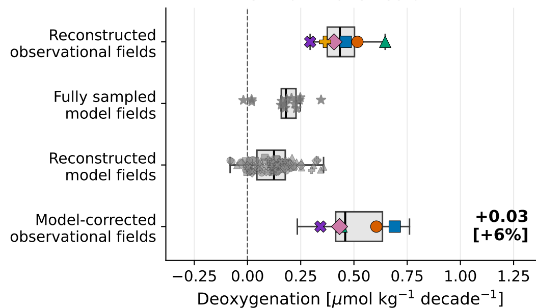
c. Full water column
