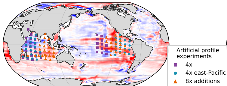
a Sampled-and-mapped - Fully-sampled trend: Upper 2000m
