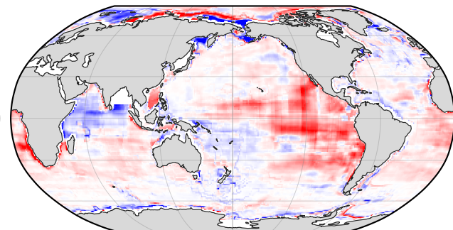
f. 2,000 added profiles: Southern Ocean
