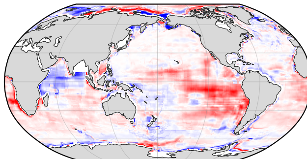
e. 2,000 added profiles: North Atlantic + North Pacific Oceans
