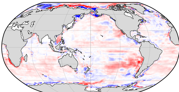
d. 2,000 added profiles: Tropical Oceans
