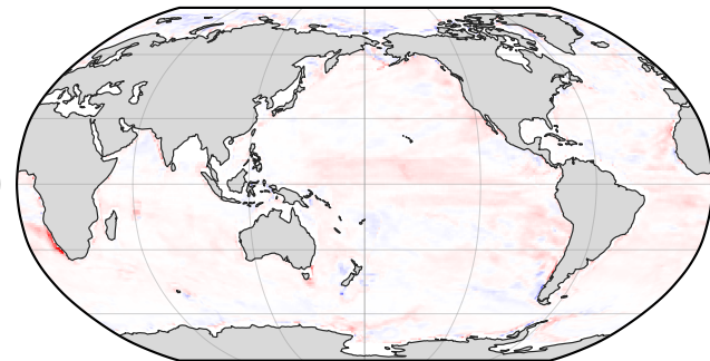
c. Uniform sampling at 30% coverage
