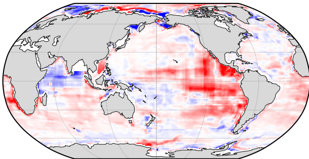
a. Historical coverage
