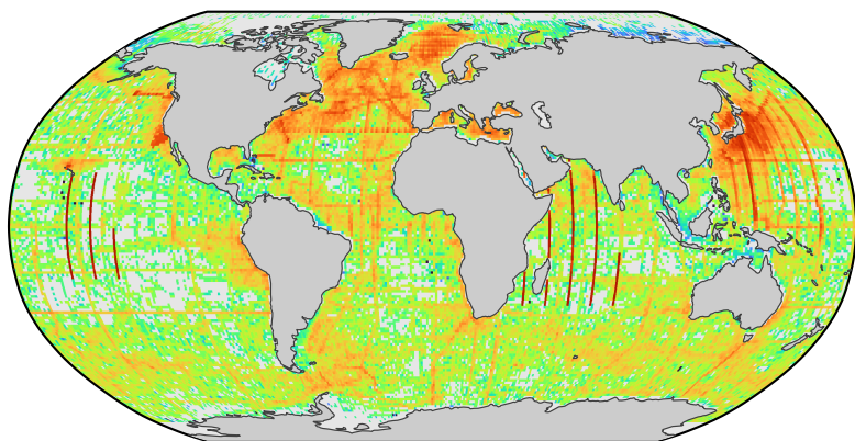
d) 4x sampling
