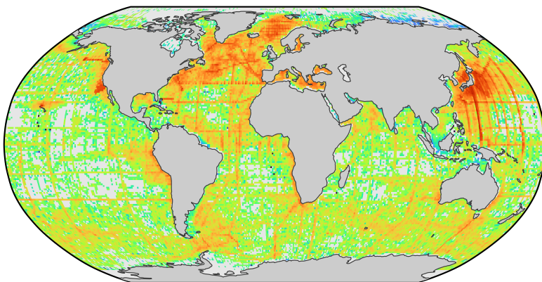
a) Original sampling
