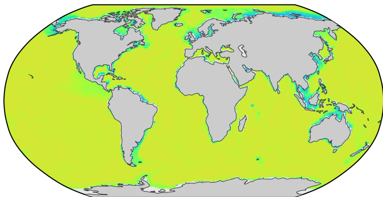
b) Randomized observed sampling
