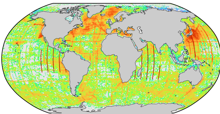
e) 4x eastern Pacific sampling
