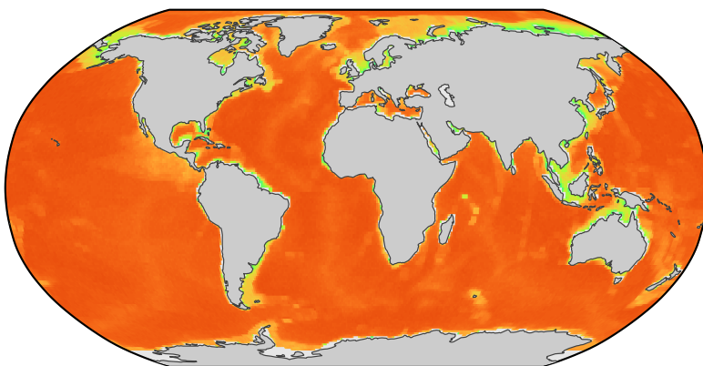
c) 30% uniform sampling
