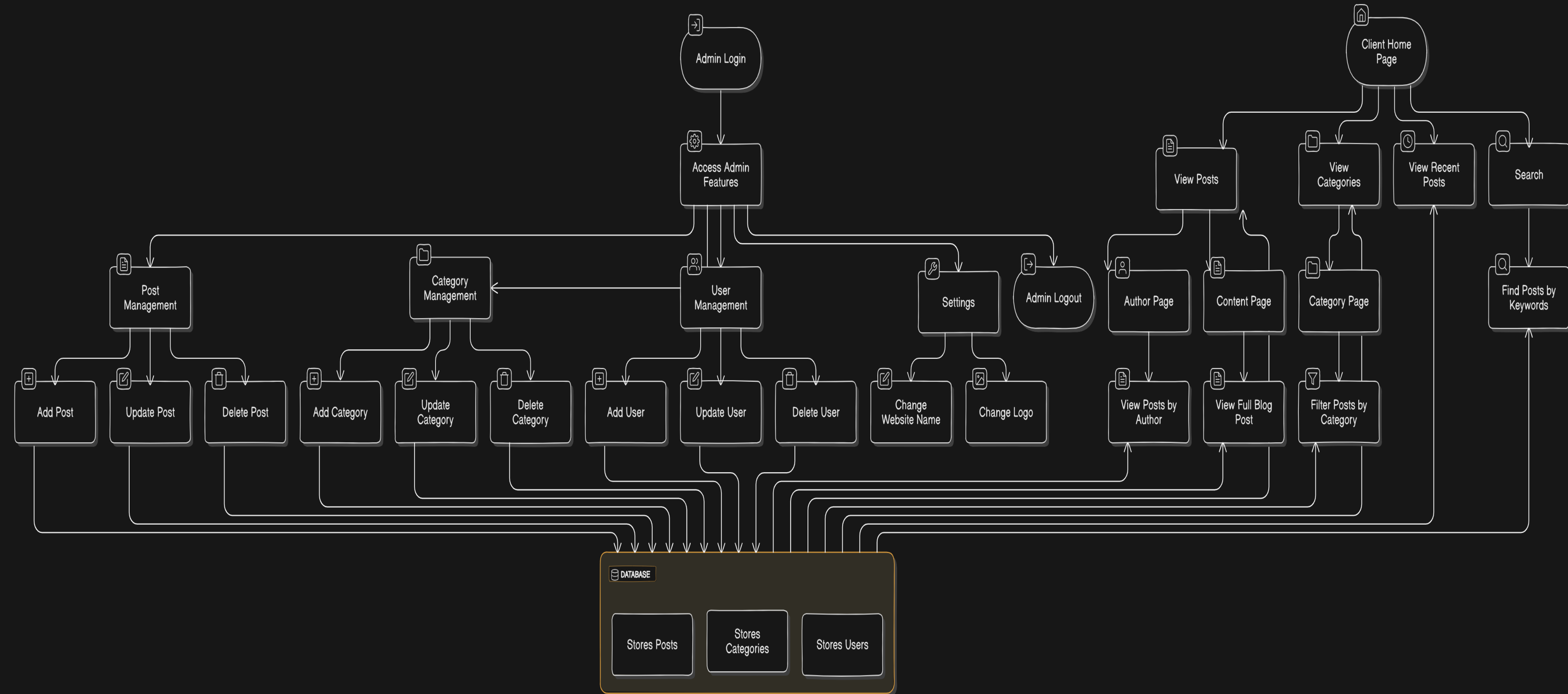
News Blogging Website Task Flow
