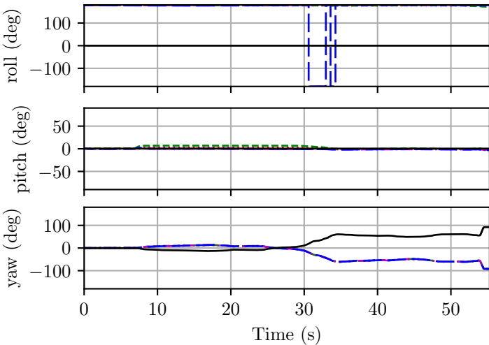
Attitude Estimation
