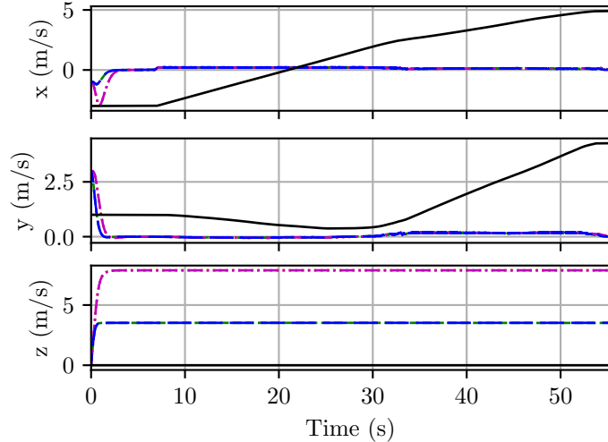
Velocity Estimation
