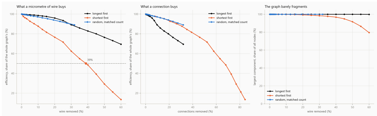
Figure 13: Efficiency against the wire removed and against the connections removed under three removal schedules, and the size of the largest weakly connected component.
