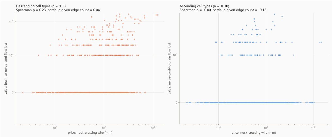
Figure 6: Price and flow value of individual descending and ascending cell types.
