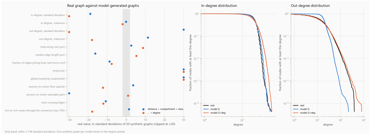
Figure 7: Thirteen properties of the real graph against 50 synthetic graphs from each generative model.
