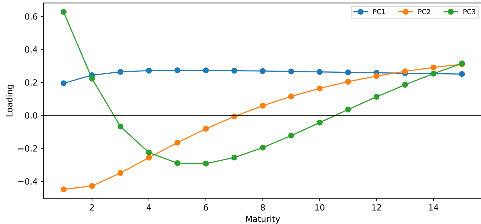
Covariance PCA loadings on daily Treasury yield changes
