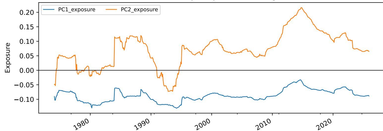
Residual level and slope exposure after regularization
