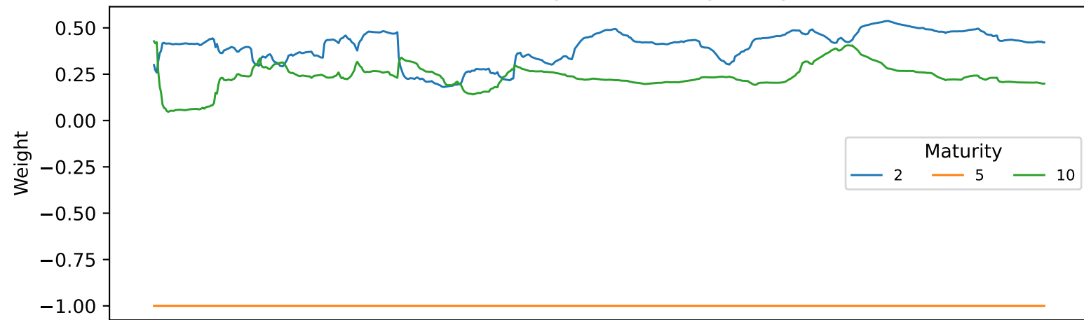
Walk-forward regularized hedge weights
