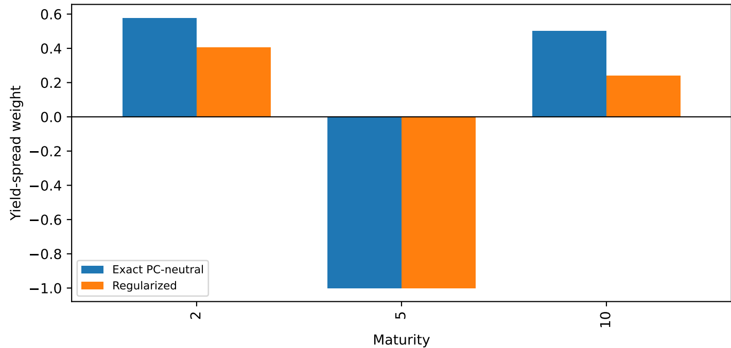
2s5s10s weights: exact neutrality versus stable hedge
