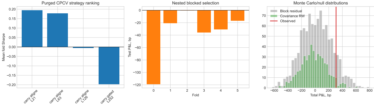
Figure 5: Robustness evidence for the Treasury RV project. The panels show purged CPCV strategy ranking, nested blocked mean-reversion selection, and block/covariance null distributions for the carry-aligned momentum branch.
