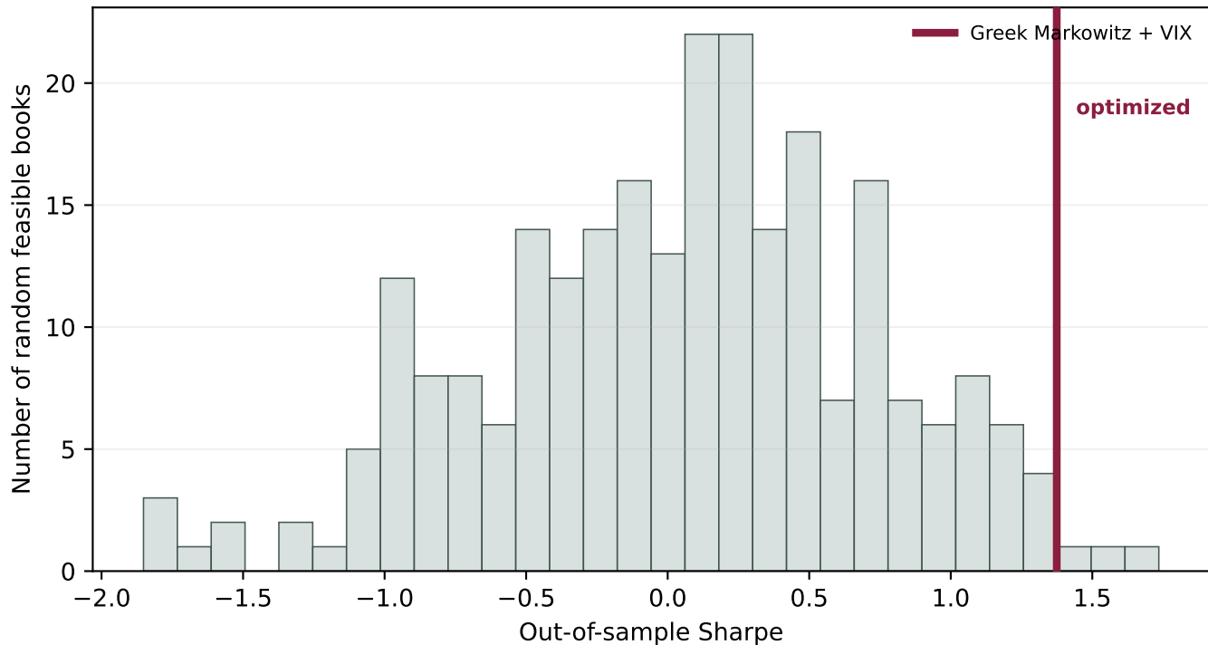
Random feasible option portfolios
