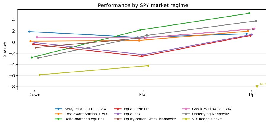
Figure 8: Sharpe ratios by SPY-return tercile. The figure visualizes Table 38. Values below -8 are clipped and annotated with the true Sharpe so that a single failed sleeve does not compress the axis.
