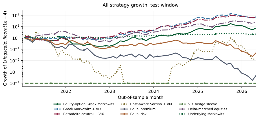
Figure 6: All-strategy out-of-sample growth diagnostic. The main text shows the central strategies; this appendix figure keeps every generated strategy visible for auditability.
