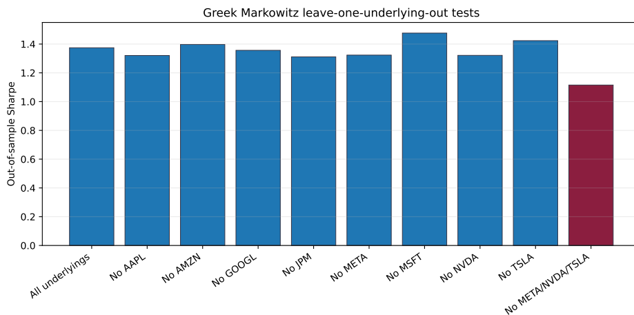
Figure 10: Out-of-sample Sharpe ratios for leave-one-underlying-out variants (Table 42).
