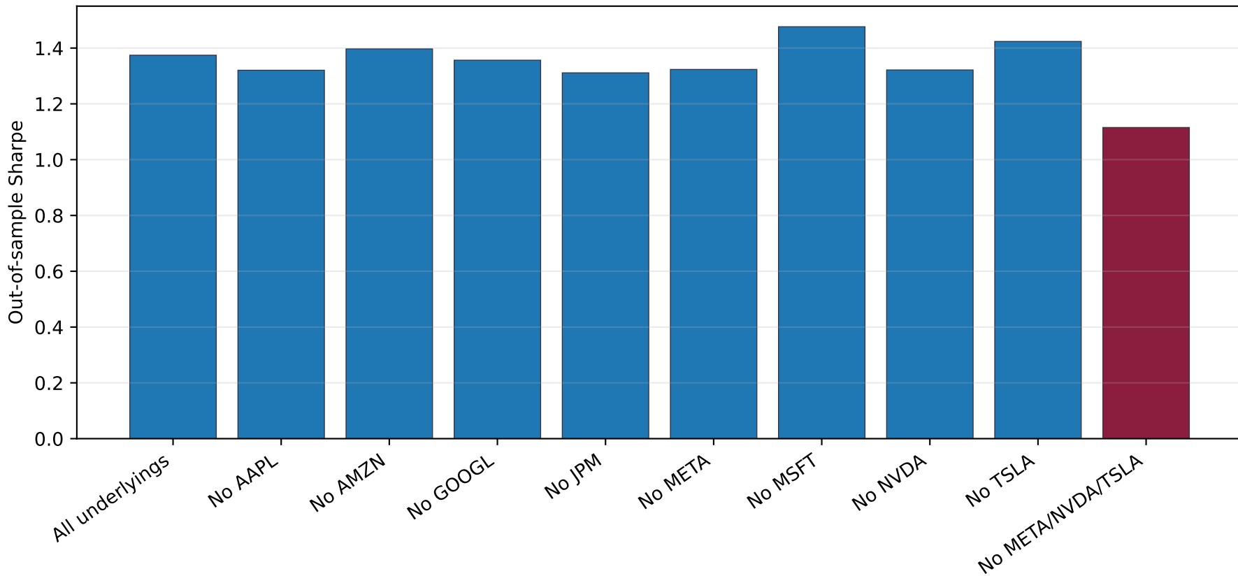
Greek Markowitz leave-one-underlying-out tests
