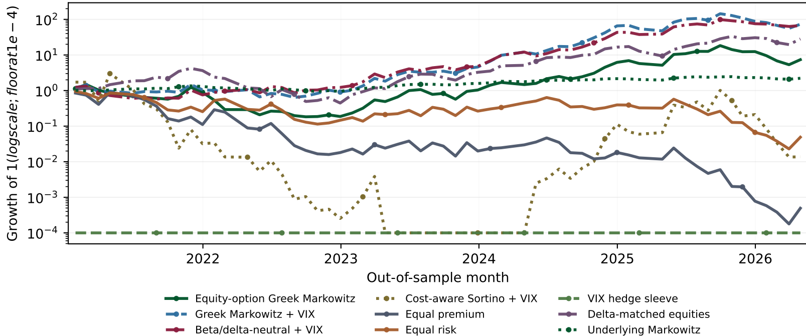
All strategy growth, test window
