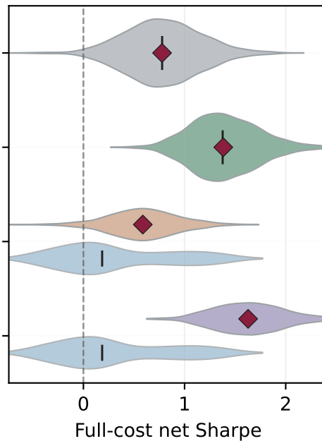
MC resampled histories
