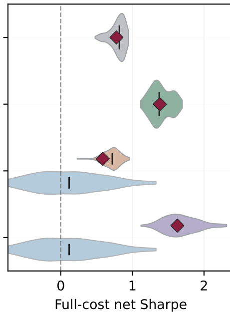
MC refit stability
