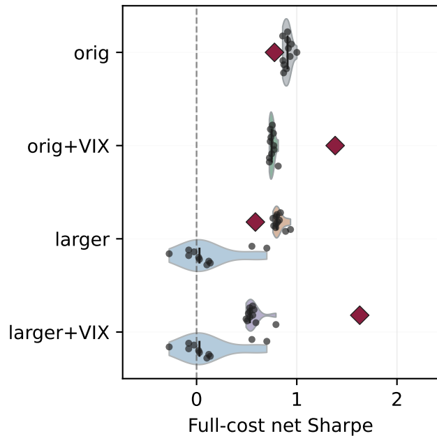
CPCV complete paths
