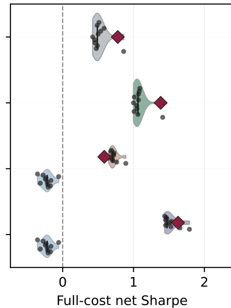
CPCV claim window
