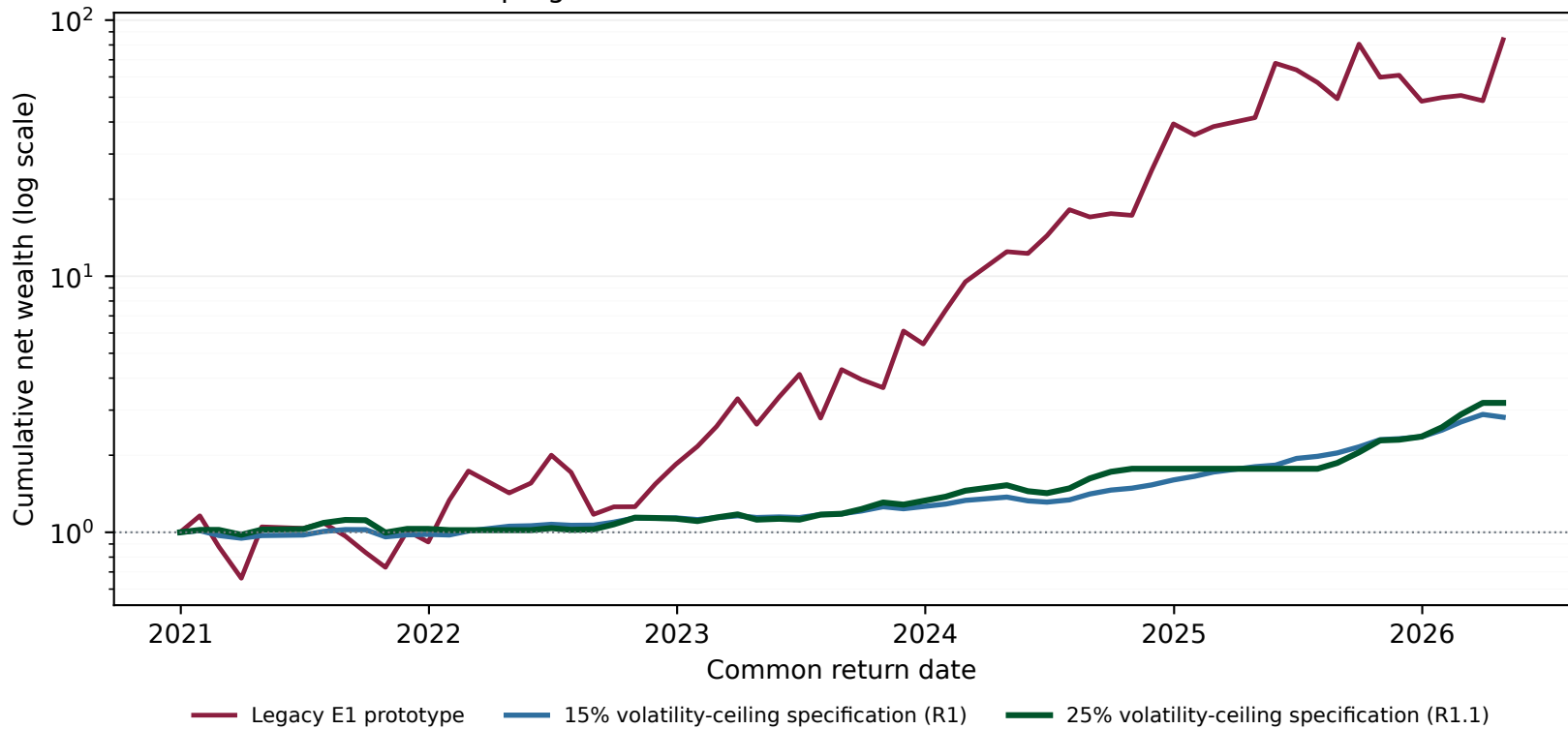
Model progression on the common 2021-2026 return window
