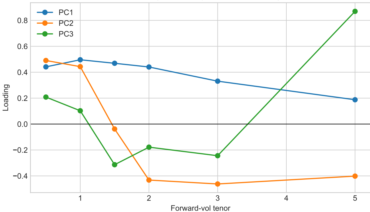
PCA loadings of weekly forward-vol changes
