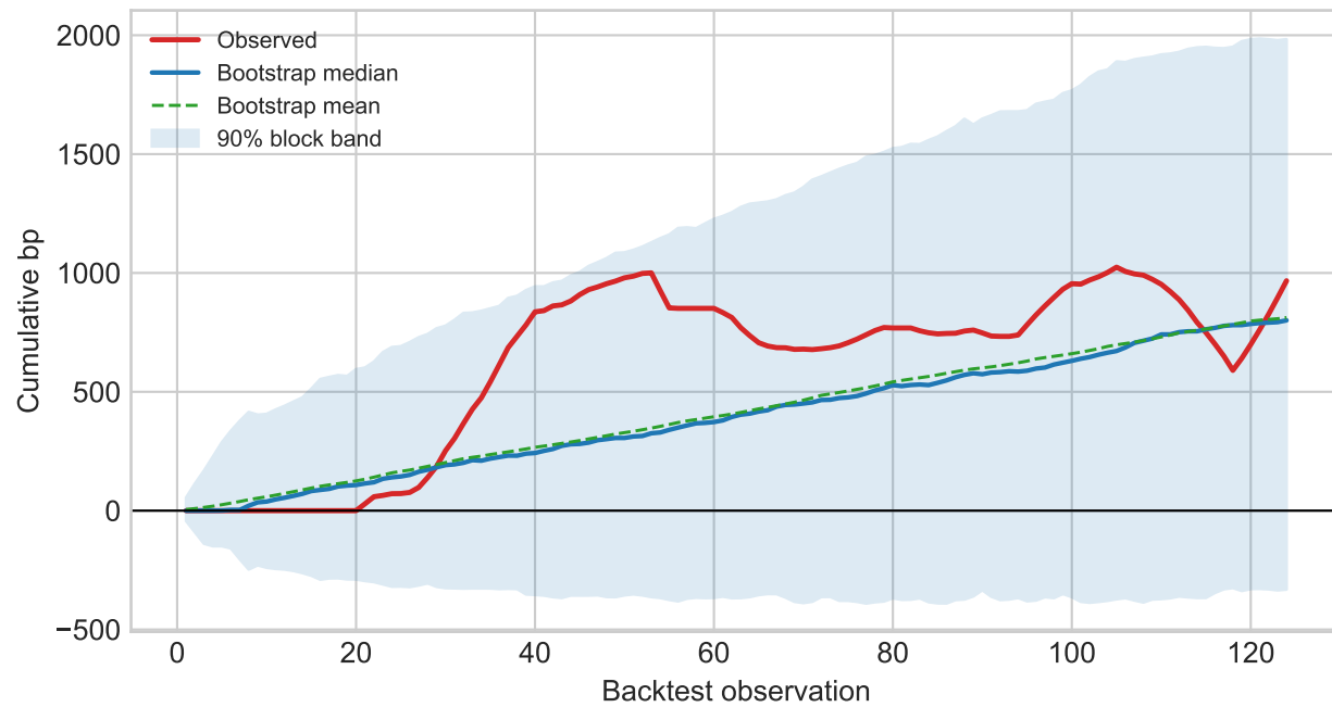
Block-bootstrap cumulative P&amp;L paths
