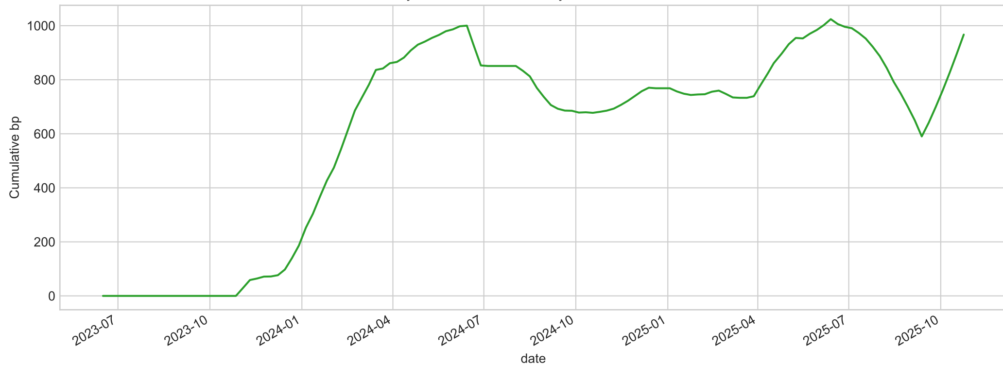
Stylized forward-vol carry P&L after costs
