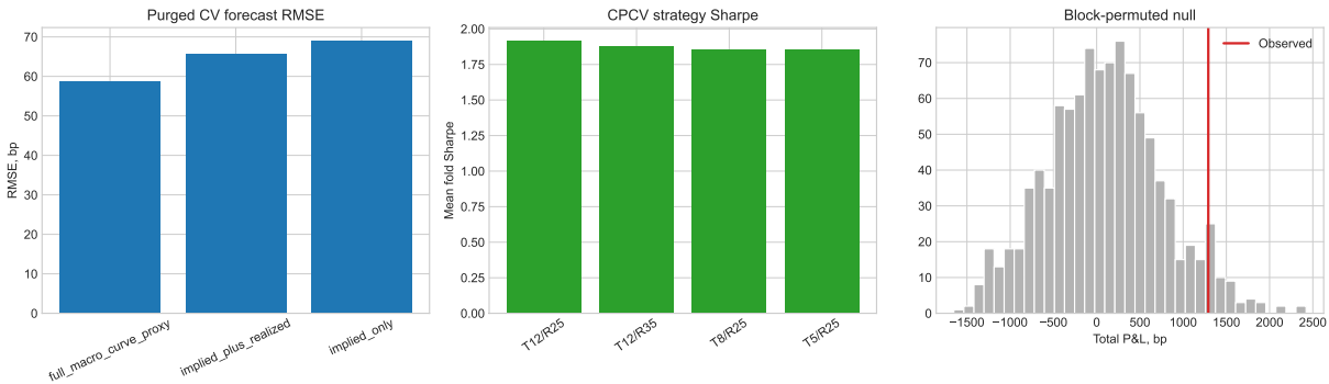
Figure 4: Robustness evidence for the SOFR rates-volatility carry screen. The panels show purged forecast-CV RMSE by feature set, CPCV strategy Sharpe for pre-declared configurations, and a block-permuted null distribution for total P&L.
