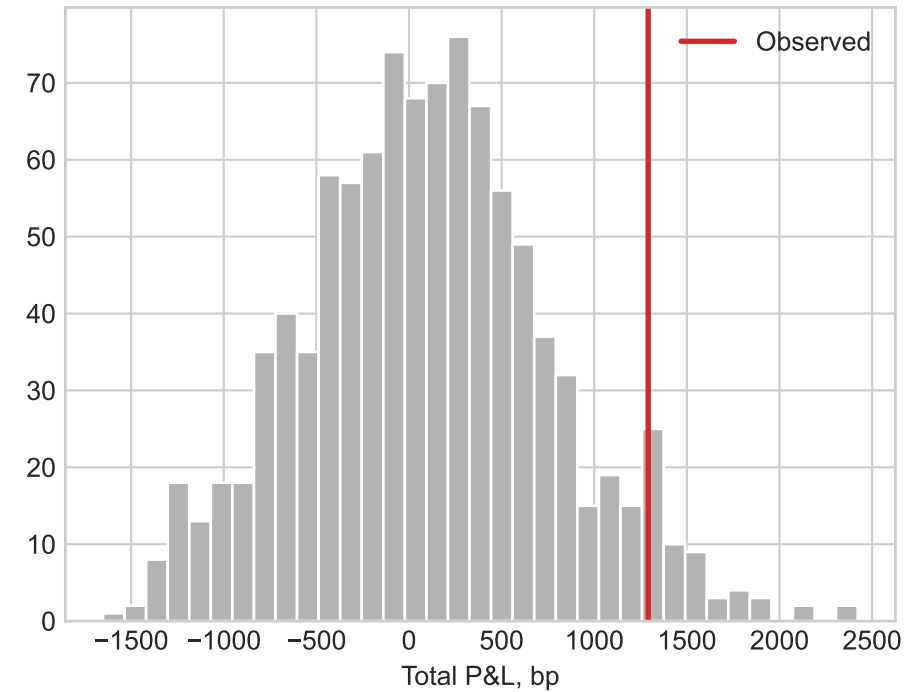
Block-permuted null
