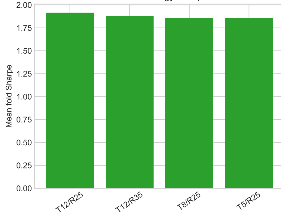
CPCV strategy Sharpe
