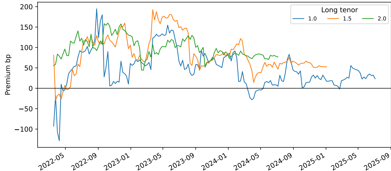
Forward-vol term premium versus future 0.5Y forward vol
