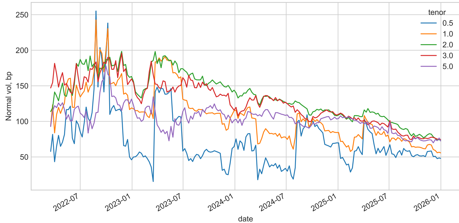
Stripped SOFR caplet forward normal vols
