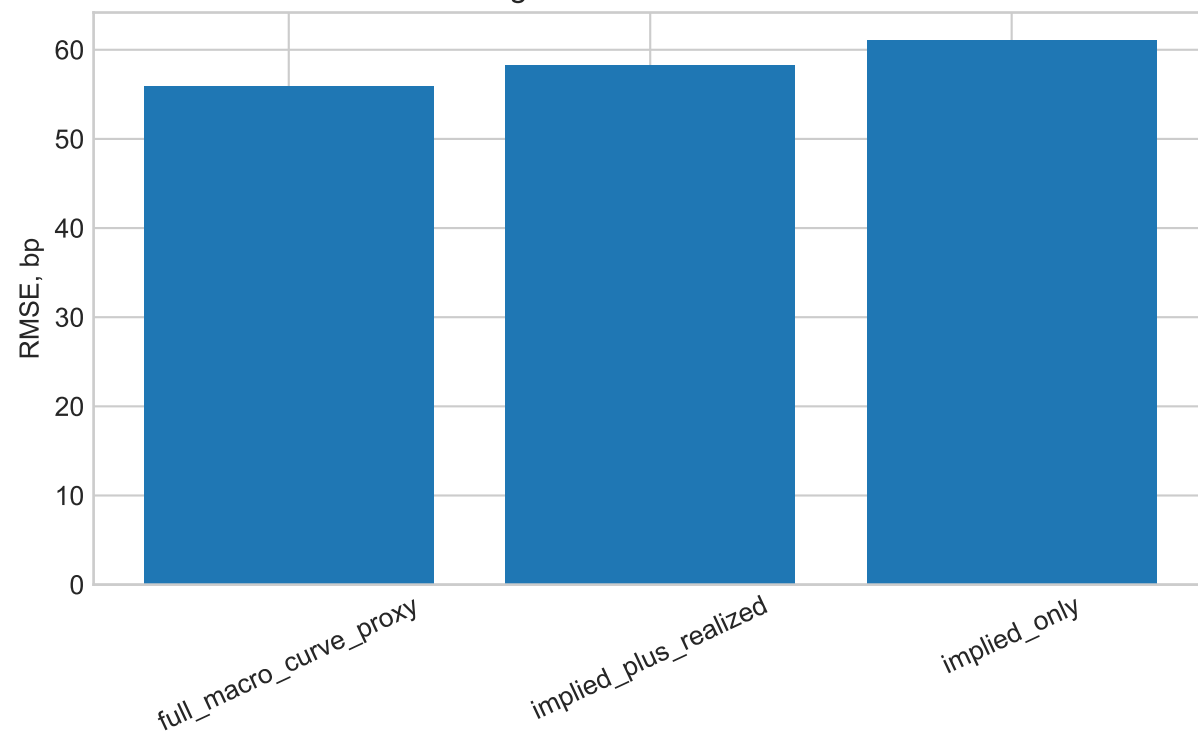
Block-permuted null
