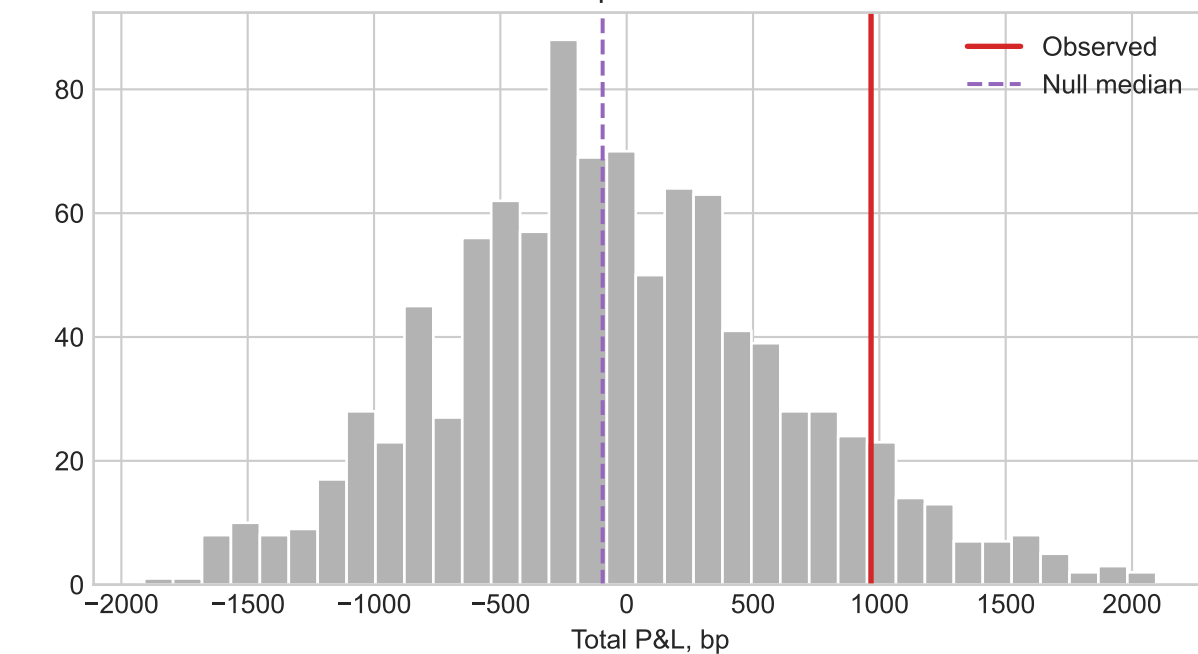
Block-permuted null
